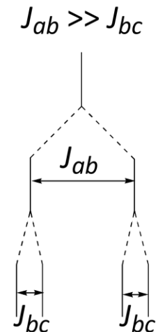
Doublet de doublets
